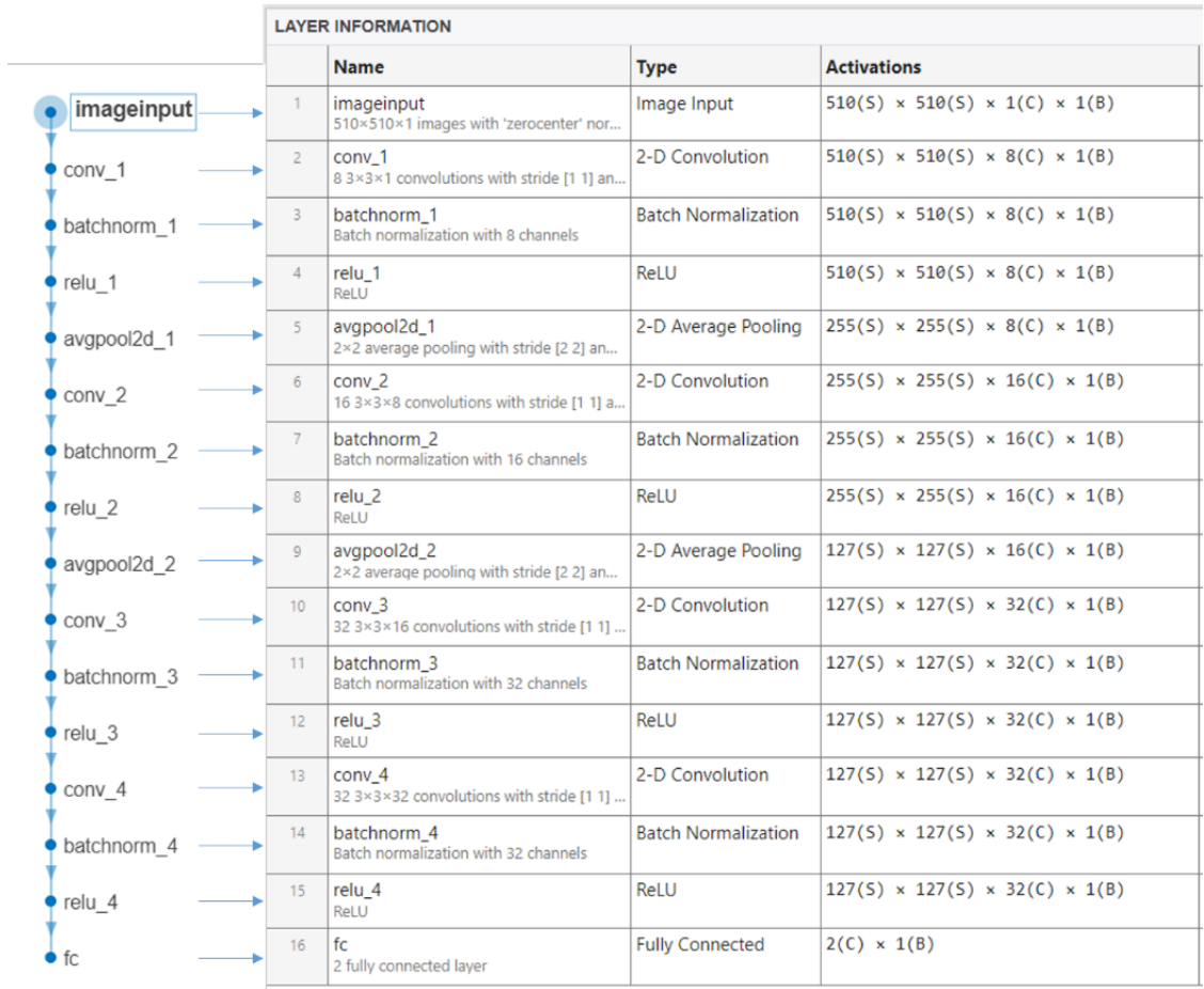
Fig. 8. Details of the architecture of the convolutional neural network model
