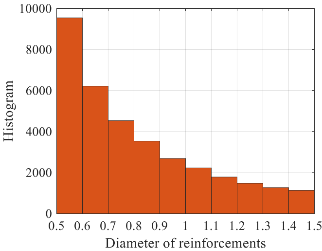
Fig. 6. Histogram of the diameter of reinforcements
