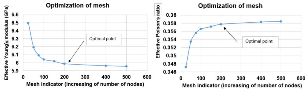
Fig. 3. Optimization of the number of nodes in the finite element domain for both effective Young's modulus and Poisson's ratio of the composite
