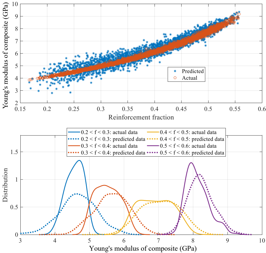
Fig. 11. Sensitivity analysis for different ranges of Young's modulus of the composite
