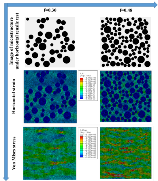
Fig. 2. Examples of 2 random microstructures with strain and stress fields, under a horizontal tensile test
