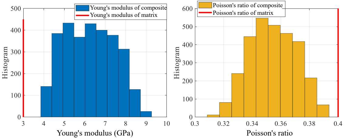
Fig. 7. Histogram of Young's modulus and Poisson's ratio of composite obtained from the finite element model (the figures also indicate the modulus of pure matrix)
