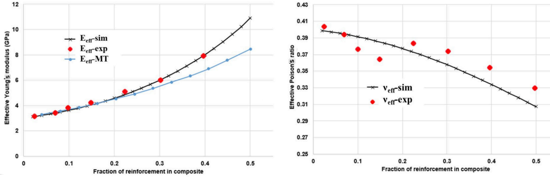
Fig. 4. Comparison of effective Young's modulus and Poisson's ratio, between the finite element model and experiments [1,2] (the Mori–Tanaka estimation is also indicated for the case of effective Young's modulus) (sim denotes the modulus from finite element simulation, exp denotes the modulus from experimentation and MT denotes the modulus from the Mori–Tanaka method)
