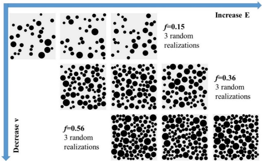
Fig. 5. Illustration of different random microstructures, in increasing the reinforcement fraction f
